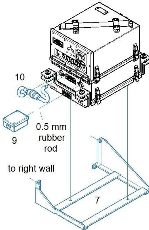
main radio set of the vehicle parts 1 & 15
